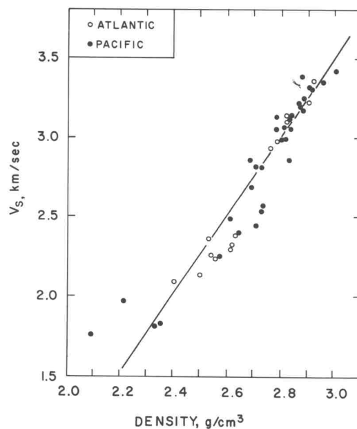
Fig. 3. Shear wave velocity ( V_s ) vs. density ( \rho ) at 0.5 kb for layer 2 basalts.
